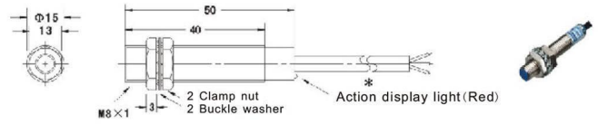
Chart 36 LJ8A3-1-□
