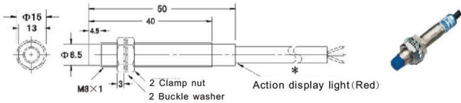
Chart 37 LJ8A3-2-□
