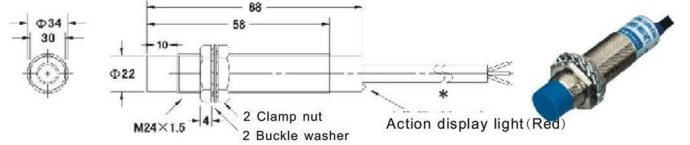
Chart 44 LJ24A3-10-□
