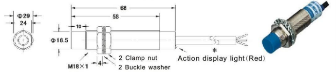
Chart 42 LJ18A3-8-□
