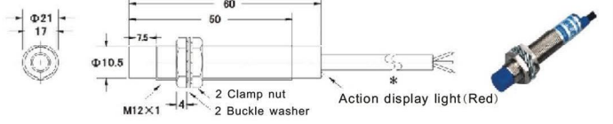
Chart 40 LJ12A3-4-□
