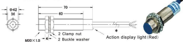
Chart 45 LJ30A3-10-□
