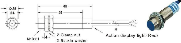
Chart 41 LJ18A3-5-□
