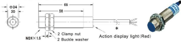
Chart 43 LJ24A3-8-□
