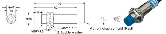
Chart 46 LJ30A3-15-□
