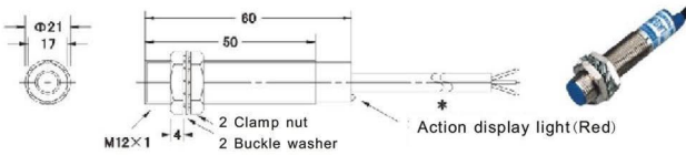
Chart 39 LJ12A3-2-□
