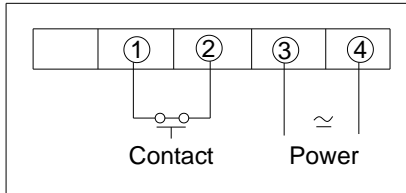
Contact input
