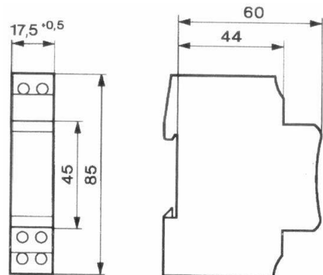
Dimension
