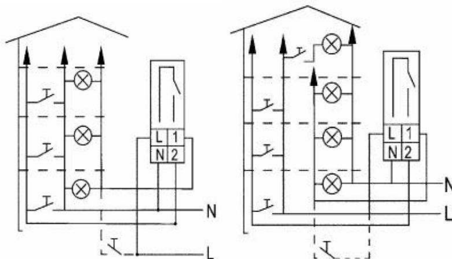
Wiring diagram
